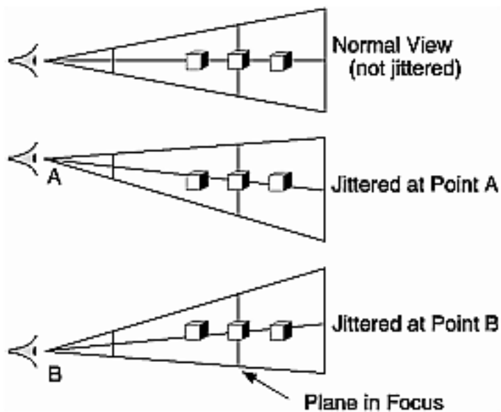
Figure 10-3 Jittered Viewing Volume for Depth-of-Field Effects
