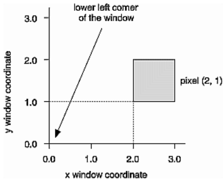
Figure 10–1 Region Occupied by a Pixel
